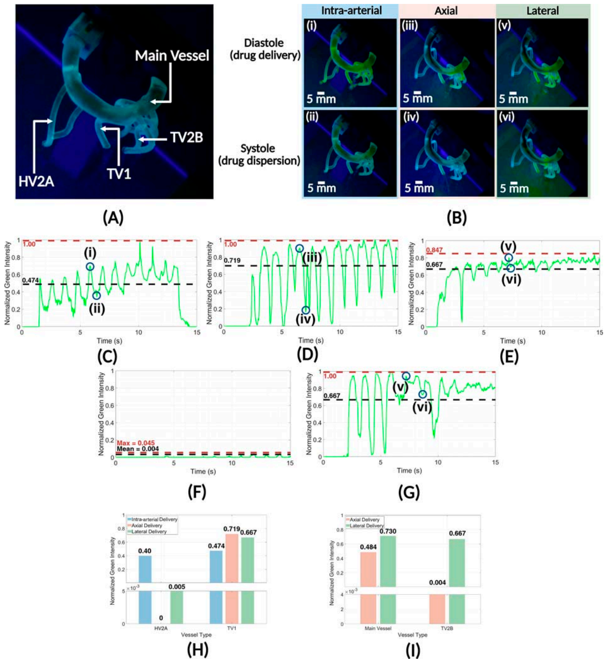
FIG. 10. Fluorescent distribution profiles, time series, and comparative profiles for intra-arterial, axial, and lateral C-MSCR delivery cases throughout diastolic and systolic phases, (A) phantom reference with annotated vessels in correspondence with main intensity analysis points throughout delivery, (B) diastolic and systolic fluorescence profiles throughout the fifth delivery pulse. (C) intra-arterial delivery at TV1, (D) axial C-MSCR delivery at TV1, (E) lateral C-MSCR delivery at TV1, (F) axial \mu -channel delivery at TV2B, (G) lateral \mu -channel delivery at TV2B, (H) comparison of intra-arterial (blue), axial (peach), and lateral (green) mean intensities in HV2A and TV1 over 15 s, and (I) comparison of axial (peach) and lateral (green) mean intensities in the main vessel and TV2B over 15 s. C-MSCR, conical tapered magnetic soft continuum robot. Created in BioRender with appropriate permissions for use. Bacchetti, A. (2026) https://BioRender.com/zqz539p .
