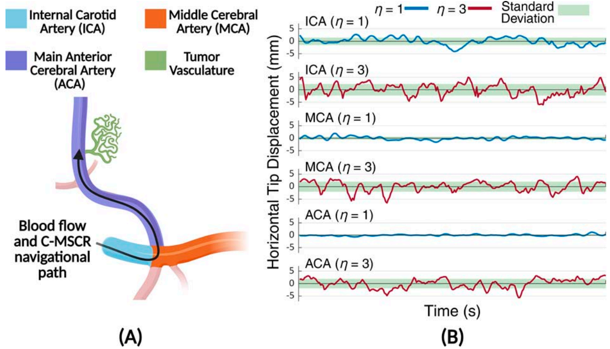
FIG. 7. Comparison of horizontal oscillatory tip displacement for \eta = 1 and \eta = 3 designs under ICA, MCA, and ACA pulsatile flow conditions. (A) Labeled diagram of blood flow direction and cerebral vessels navigated throughout SSIACI, and (B) horizontal oscillatory tip displacements for \eta = 1 (blue) and \eta = 3 (maroon) designs with associated standard deviations (green shading), under respective vessel flow conditions. ACA, anterior cerebral artery; ICA, interior carotid artery; MCA, middle cerebral artery; SSIACI, superselective intra-arterial cerebral infusion. Created in BioRender with appropriate permissions for use. Bacchetti, A. (2026) https://BioRender.com/qhaeyeq .
