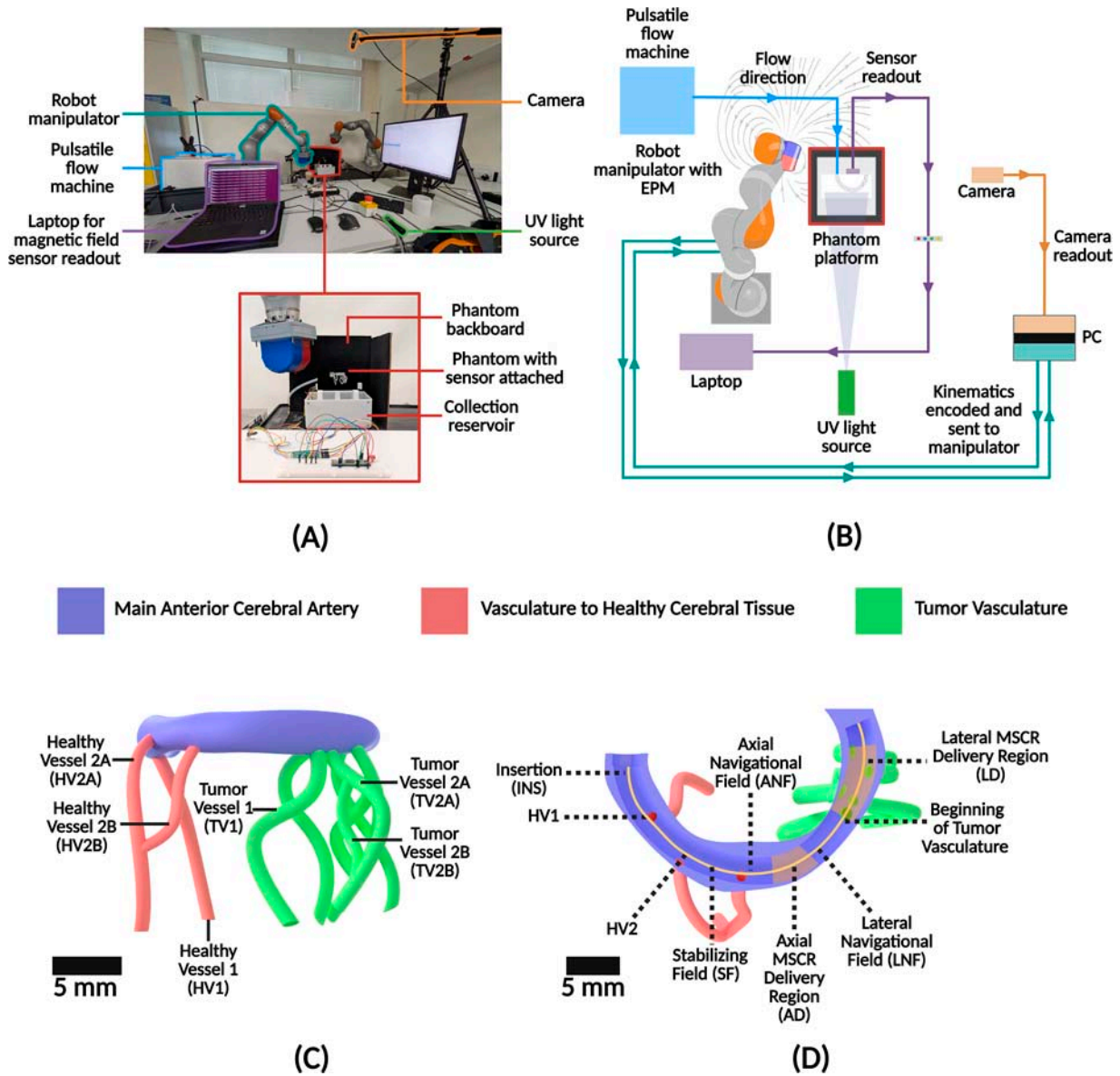
FIG. 8. Experimental setup and color coded neurovascular flow phantom, (A) phantom experiment setup with key apparatus with expanded view of phantom rig, (B) systematic diagram highlighting equipment interactions and information flow, (C) phantom diagram of the main ACA vessel (purple) alongside branching vasculature to healthy peripheral cerebral tissue (red) and vasculature supplying a tumor (green), highlights key reference vessels for analysis and comparison of fluorescence intensity throughout traditional intra-arterial, axial and lateral \mu -channel delivery, and (D) C-MSCR navigational path from insertion to \mu -channel delivery, annotated with key reference points for fluorescent intensity, magnetic field application, and C-MSCR stabilization throughout navigation and delivery. C-MSCR, conical tapered magnetic soft continuum robot. Created in BioRender with appropriate permissions for use. Bacchetti, A. (2026) https://BioRender.com/k47ro9o .
