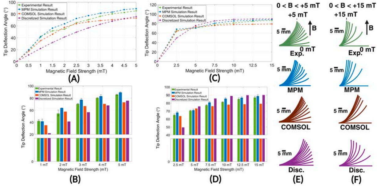
FIG. 5. Comparison of model and experimental tip deflection angle responses for cylindrical and C-MSCRs under low (0–5 mT) and high strength (0–15 mT) uniform field conditions. Error bars are presented for experimental and MPM outputs. Includes responses for experimental (green), MPM (blue), COMSOL (orange), and discretized (purple) methods, (A) tip deflection angle responses between 0 and 5 mT, (B) tip deflection angle responses between 0 and 15 mT, (C) comparison of tip deflection angle between 0 and 5 mT in 1 mT increments, with upper and lower measurement error bars, (D) comparison of tip deflection angle between 0 and 15 mT in 2.50 mT increments, with upper and lower measurement error bars strength deflection profiles, (E) experimental and model-based deflection profiles between 0 and 5 mT, and (F) experimental and model-based deflection profiles between 0 and 5 mT. C-MSCR, conical tapered magnetic soft continuum robot; MPM, material point method. Created in BioRender with appropriate permissions for use. Bacchetti, A. (2025) https://BioRender.com/eadpcqr .
