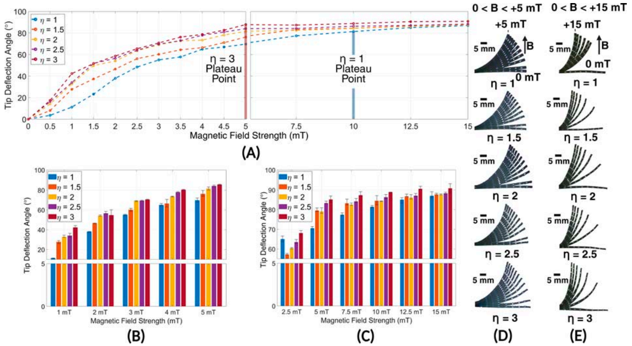
FIG. 4. Comparison of tip deflection angle for varied C-MSCR designs under low (0–5 mT) and high strength (0–15 mT) uniform orthogonal magnetic field conditions, (A) summary of tip angle deflection responses across low- and high-field strength ranges for \eta = 1 (blue), \eta = 1.5 (orange), \eta = 2 (yellow), \eta = 2.5 (purple), and \eta = 3 (maroon), with an intermediate break at 5 mT, (B) comparison of tip deflection angles at selected applied field between (B) 0–5 mT, and (C) 0–15 mT, with upper and lower measurement error bars shown. Images of MSCR deflections shown between (D) 0–5 mT, (E) 0–15 mT. C-MSCR, conical tapered magnetic soft continuum robot. Created in BioRender with appropriate permissions for use. Bacchetti, A. (2025) https://BioRender.com/gkldpuu .
